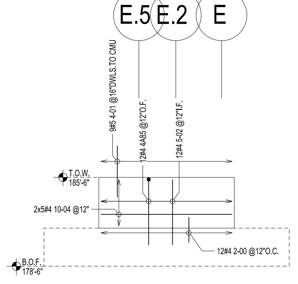
E4 CONCRETE WALL ELEVATION R104
