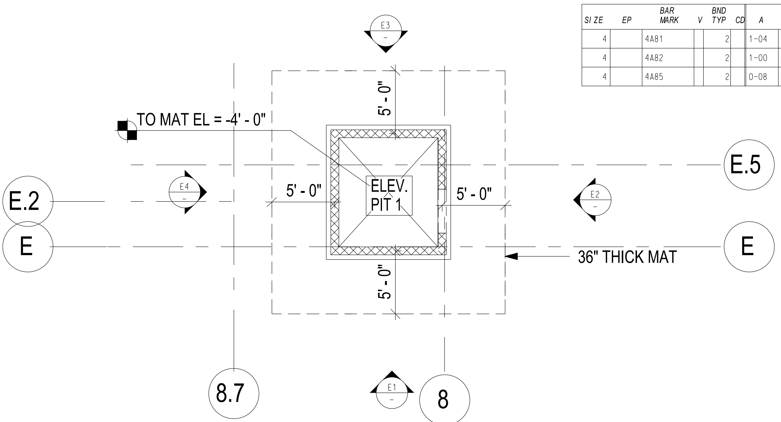
1 ELEVATOR PIT 1 PLAN R104
