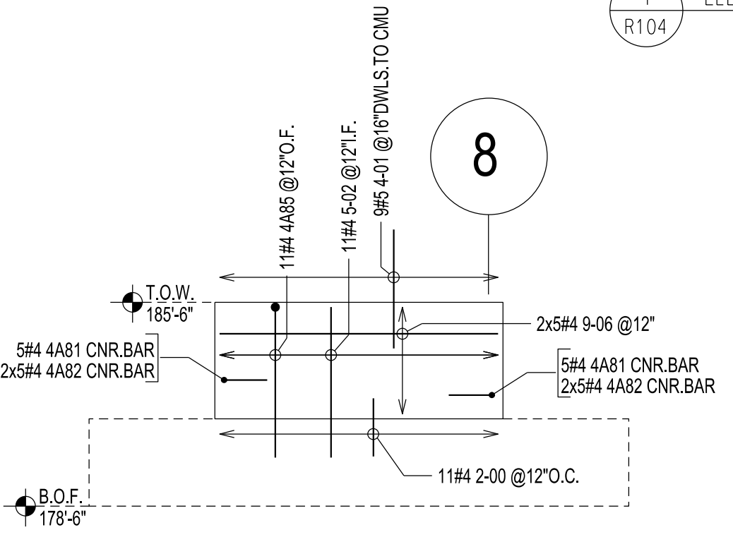
E1 CONCRETE WALL ELEVATION R104
