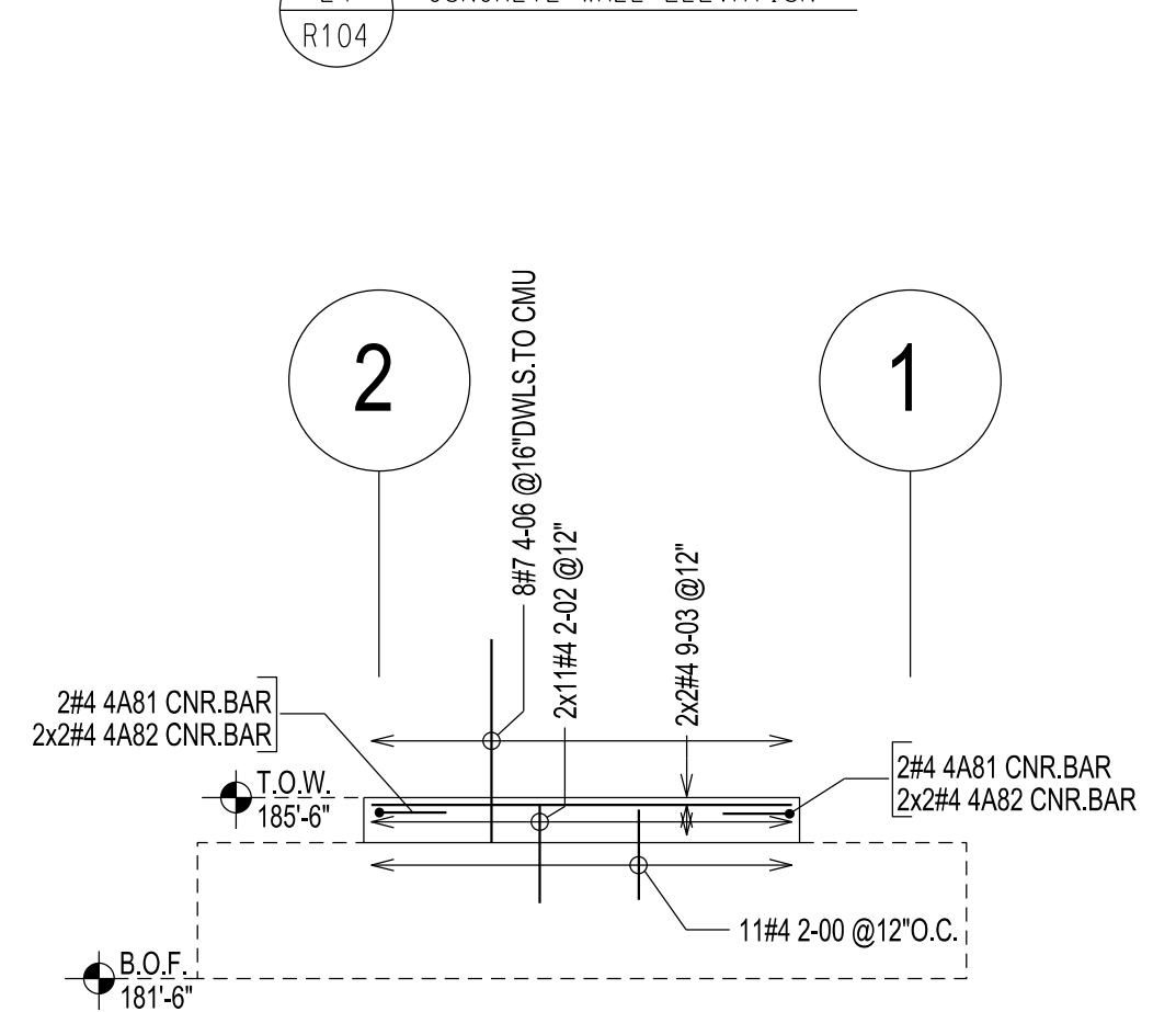
E5 CONCRETE WALL ELEVATION R104
