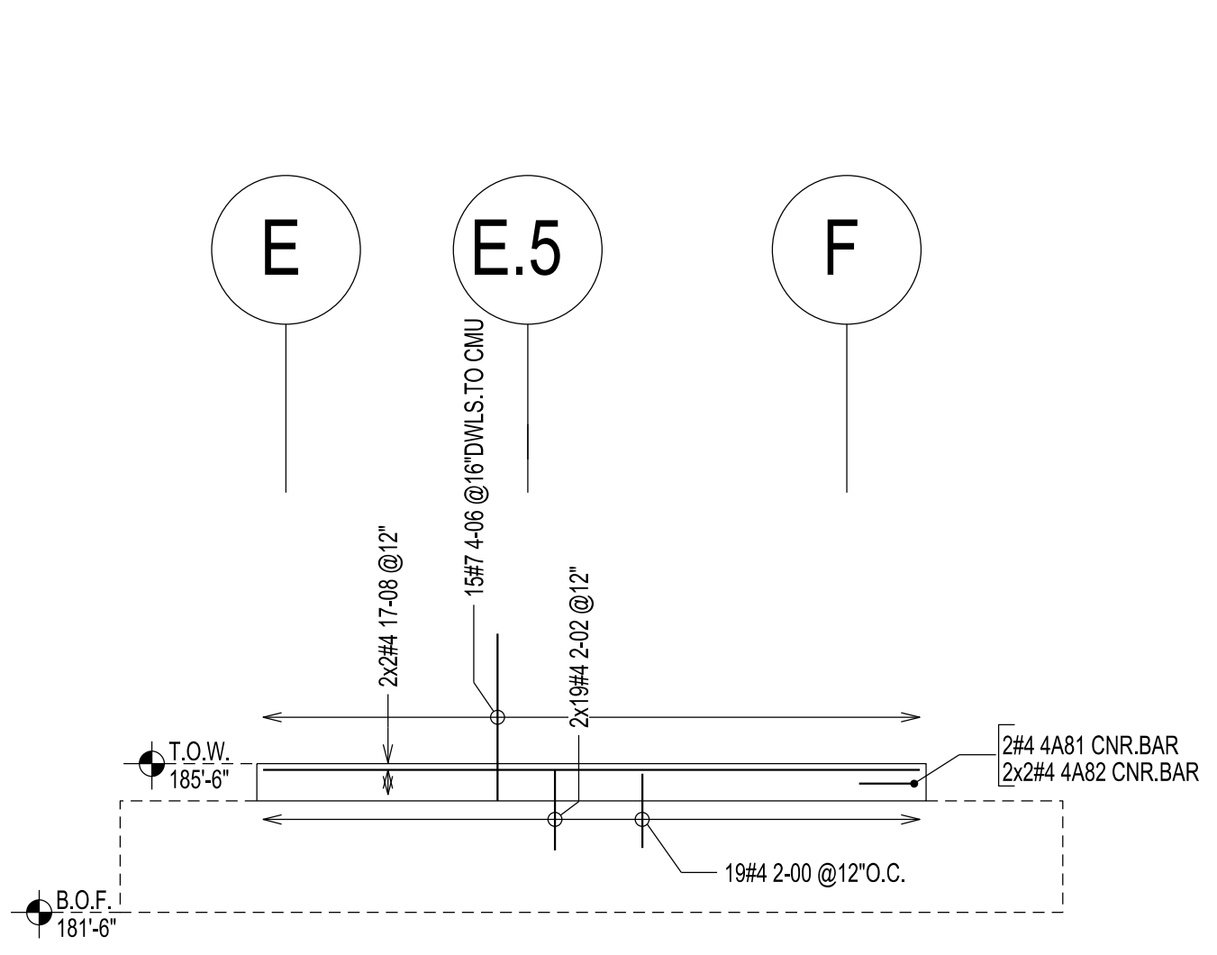
E6 CONCRETE WALL ELEVATION R104
