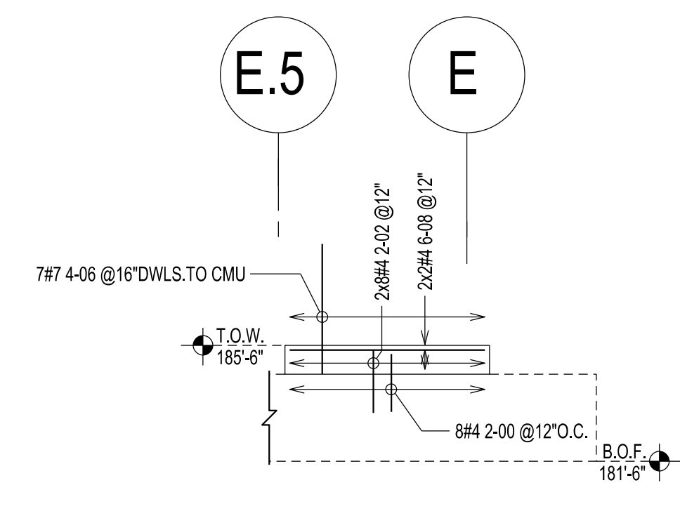
E8 CONCRETE WALL ELEVATION R104
