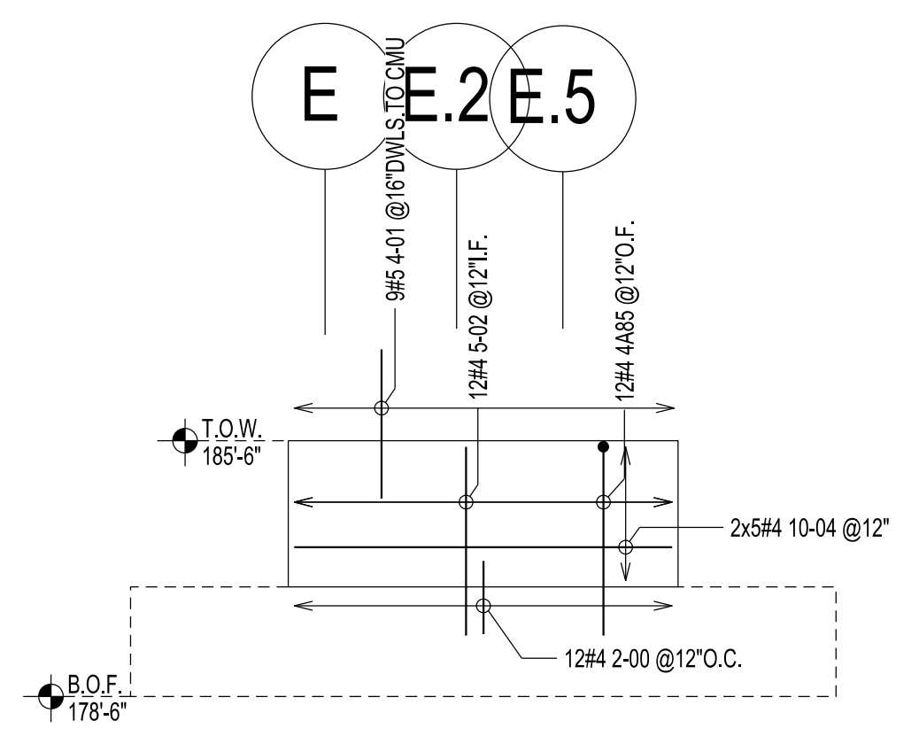
E2 CONCRETE WALL ELEVATION R104
